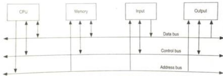
Fig.1 Microprocessor-based system
