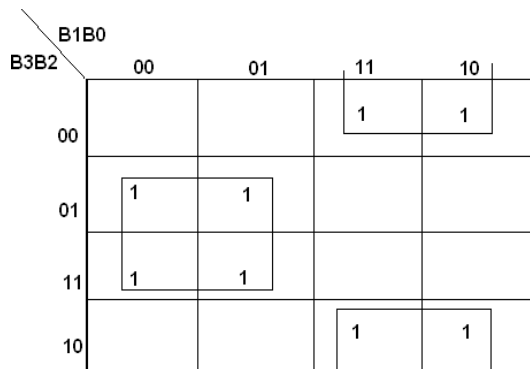
K-Map for G 1 :
