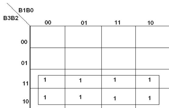
K-Map for G 3 :
