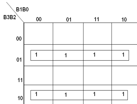
K-Map for G 2 :
