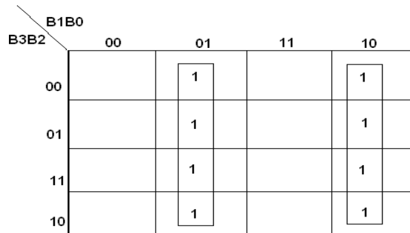
K-Map for G 0 :
